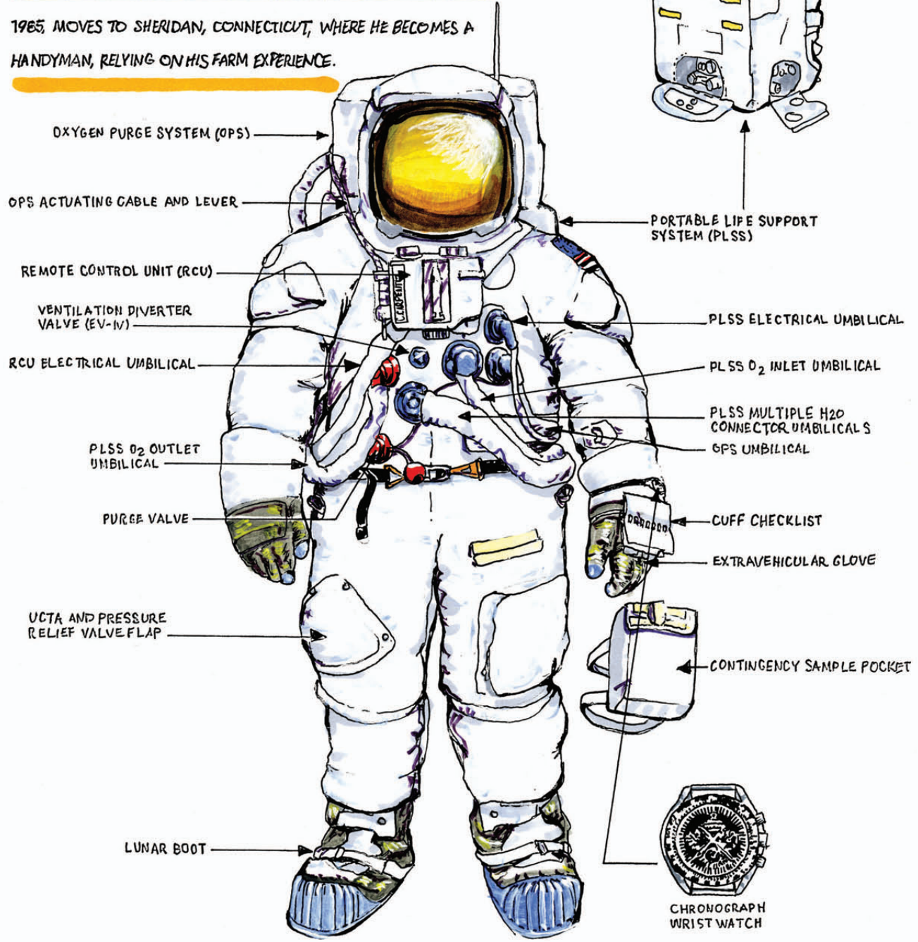
THE EXTRAVEHICULAR MOBILITY UNIT (EMU)
